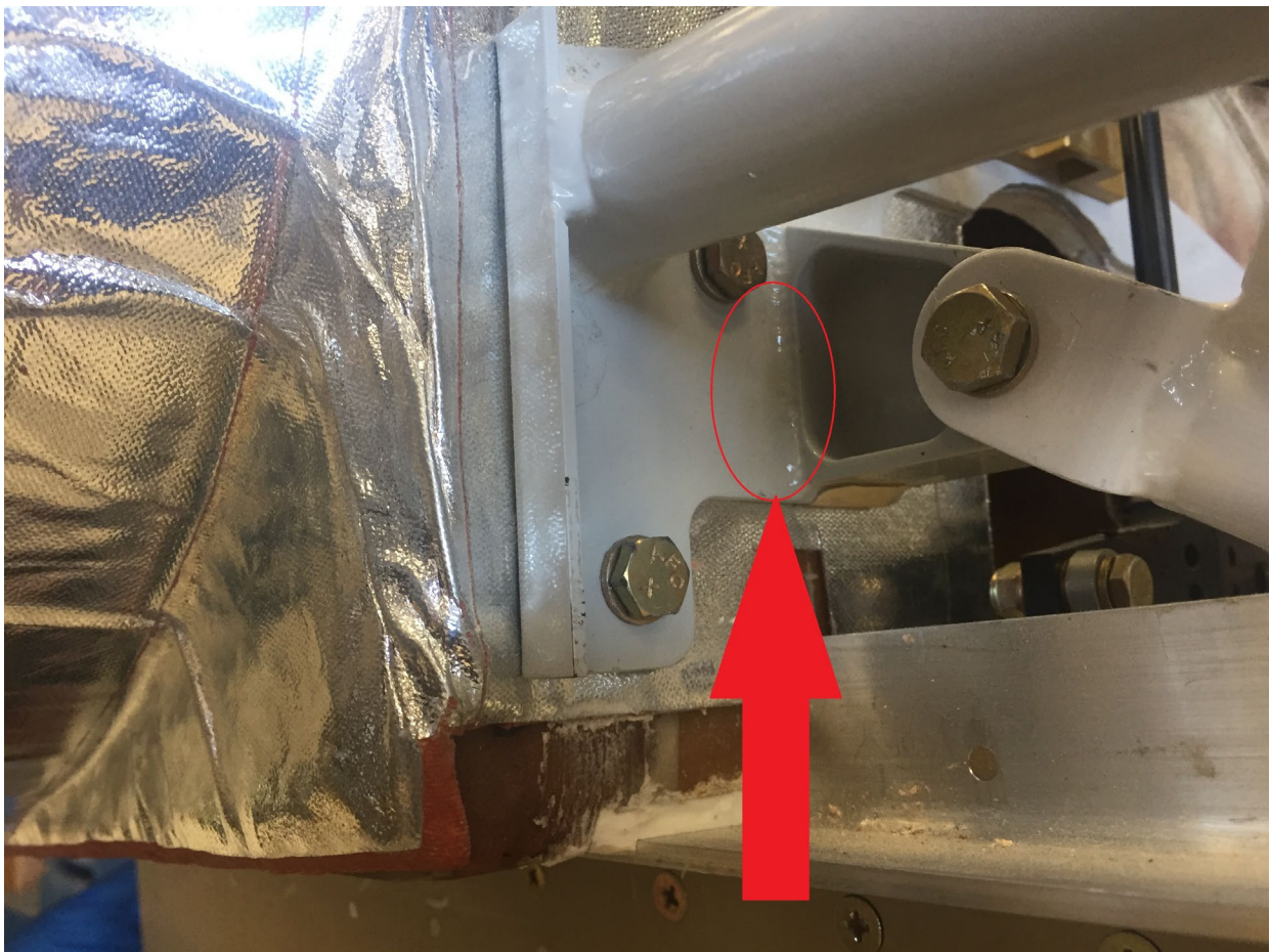
Figure 1 Original Design Lower Drag Links
